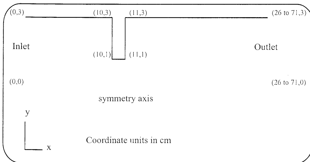
Figure 1: Two-Dimensional Axisymmetric Configuration.
