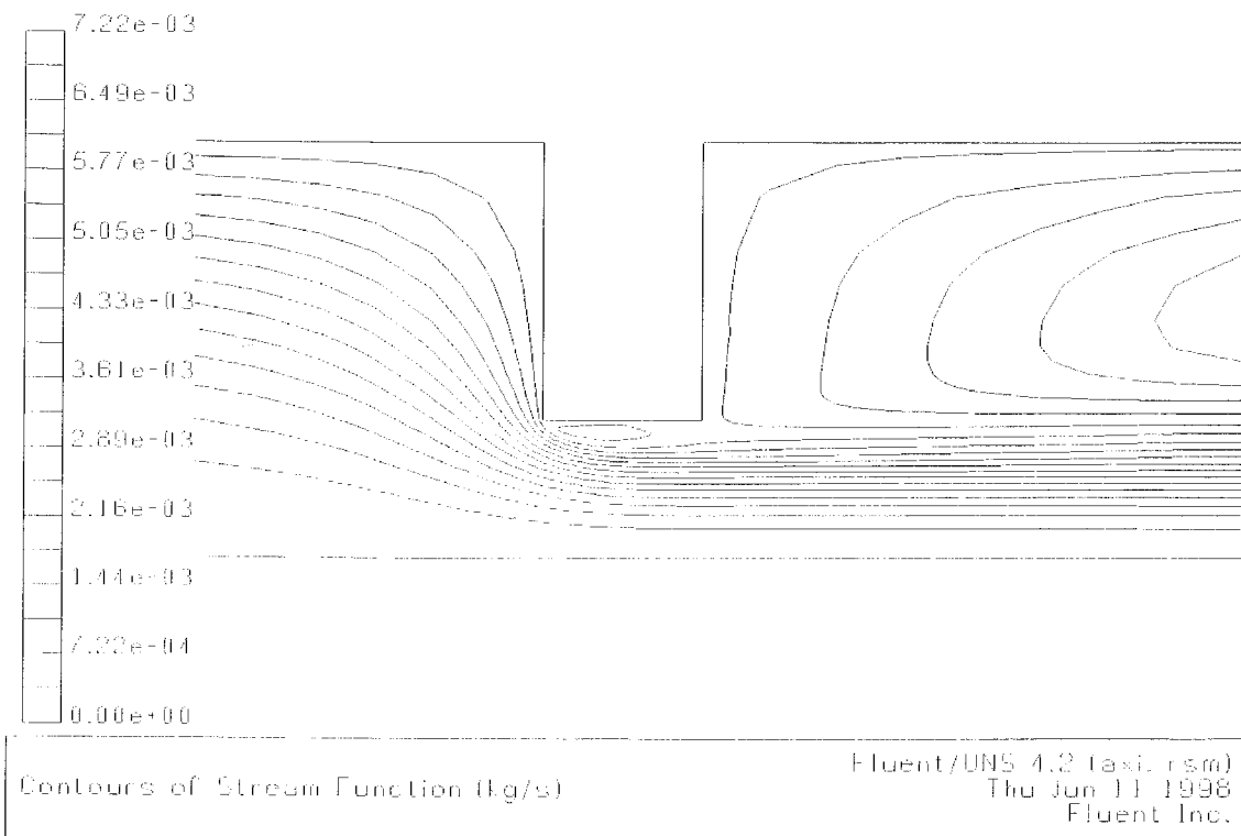
Figure 5: Streamlines of Incompressible Orifice Flow Using RSM and 3,787 Cells.
